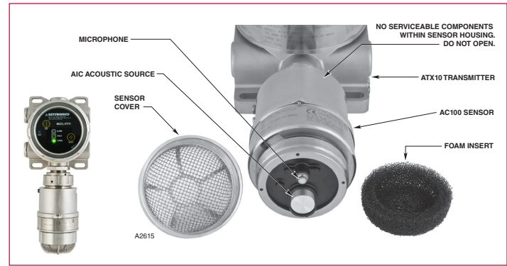
Figure 2: Acoustic gas leak detectors work by recognizing the unique sound “fingerprints” of various gases. However, the sound and impact of blowing sand particles can create nuisance ultrasonic noise and lead to possible fault conditions in windy desert environments. The Det-Tronics FlexSonic detector shown above uses a foam filter to eliminate ultrasonic noise due to particle impact with the microphone.
